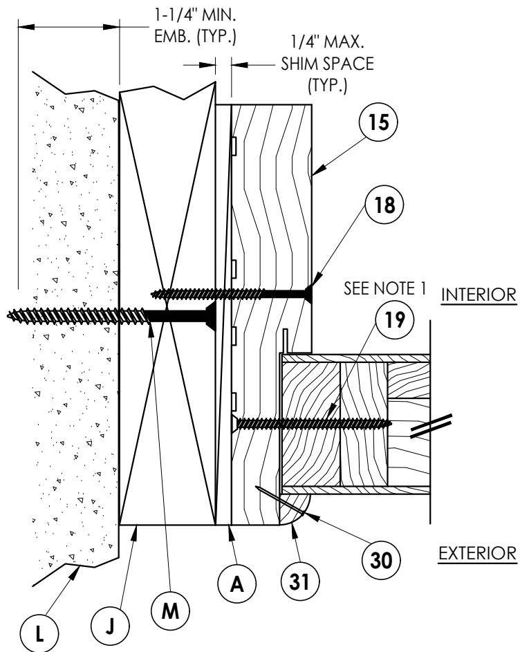
1 4 HORIZONTAL CROSS SECTION Glazed door shown - opaque door also approved Outswing shown - inswing also approved
