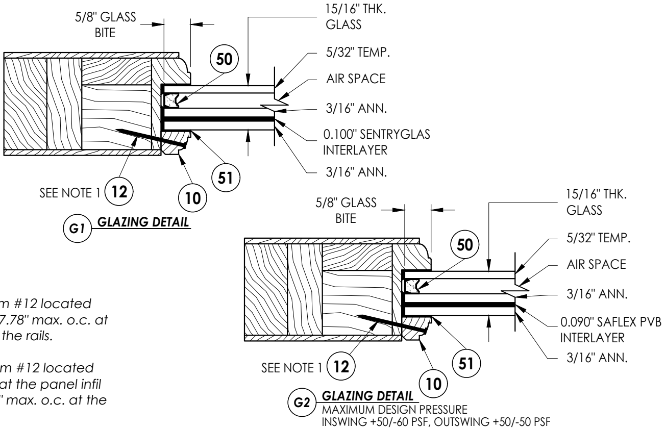
GLAZED DOOR PANEL
