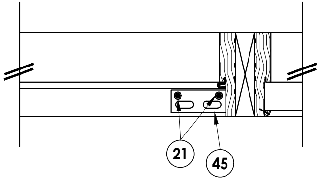
1 8 MULTI-POINT STRIKE INSTALLATION View looking up @ head
