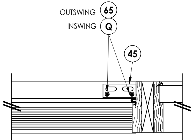
2 8 MULTI-POINT STRIKE INSTALLATION View looking down @ sill
