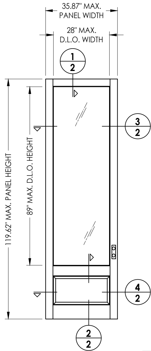
GLAZED DOOR PANEL
