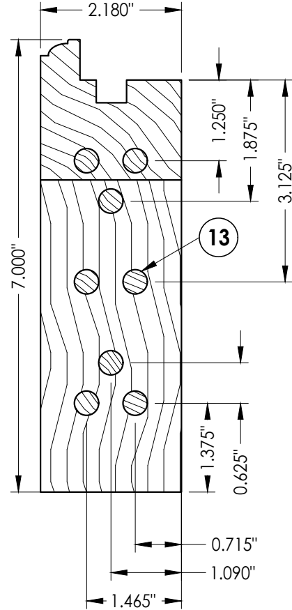
9 BOTTOM RAIL Glazed door
